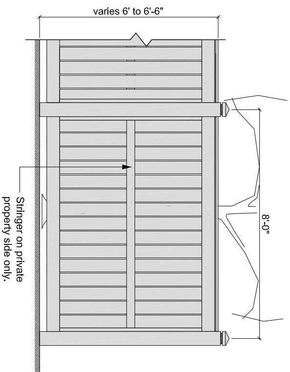
1 Solid Fence Elevation - Typ. 6C Solid Fence Design - NTS
